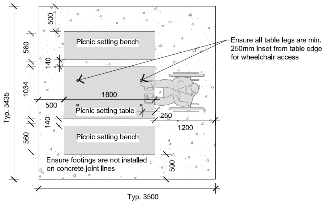
02 PARK PICNIC SETTING LAYOUT Plan View 1:50
