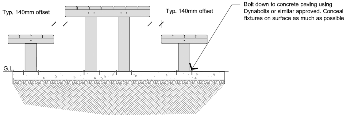
01 PARK PICNIC SETTING Front Elevation 1:25
