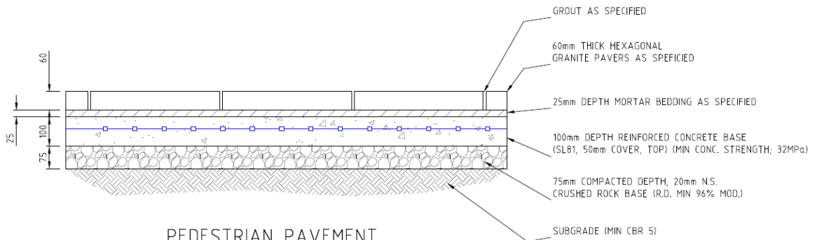
PEDESTRIAN PAVEMENT NOT TO SCALE
