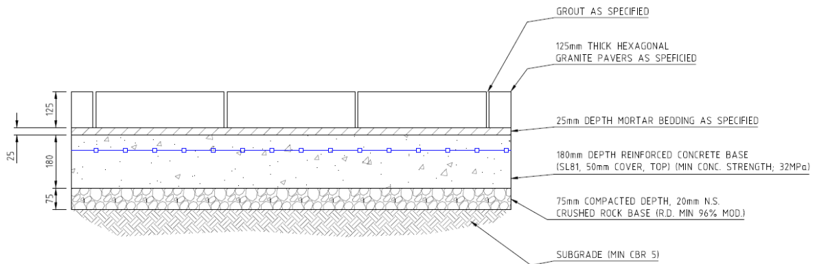
VEHICLE TRAFFICABLE PAVEMENT NOT TO SCALE
