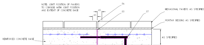
EXPANSION JOINT NOT TO SCALE
