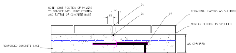
MOVEMENT JOINT NOT TO SCALE
