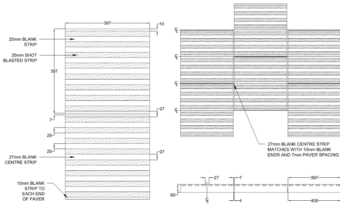
Paver Design and Spacing
